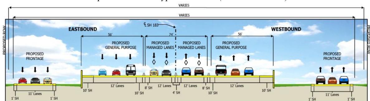
Proposed Phase 2 Typical Section (SH 161 to I-35E)
