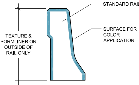
Figure 3.2 – Required aesthetic surface treatments on rails
