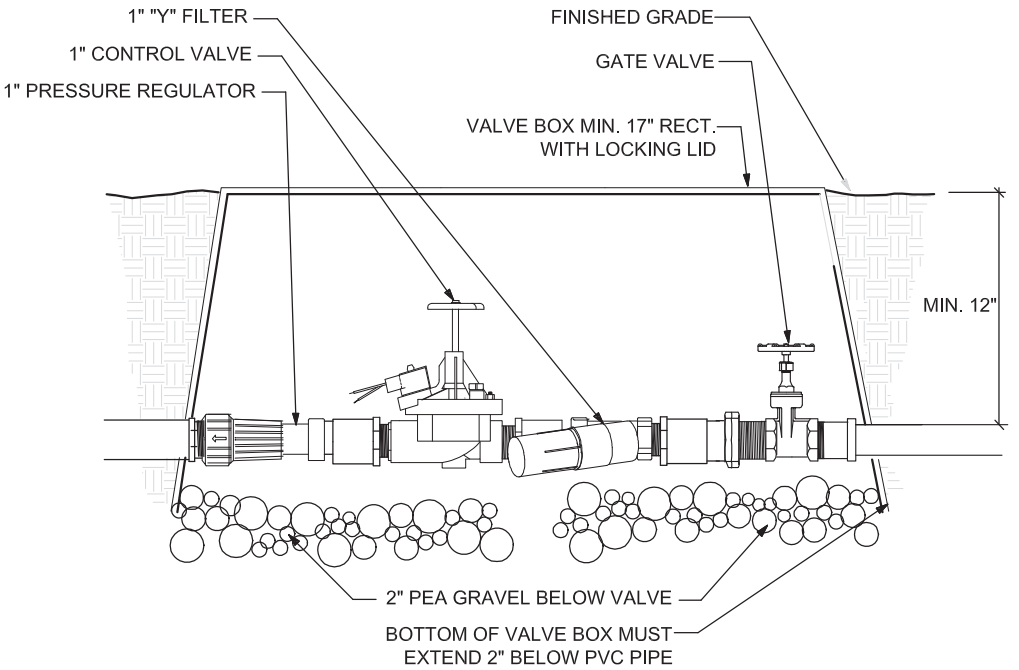
Figure 10.6 – Typical valve assembly for drip irrigation
