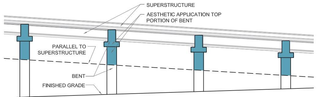
Figure 4.4 – Bents in a sloping condition with aesthetic treatment justified at the top.
