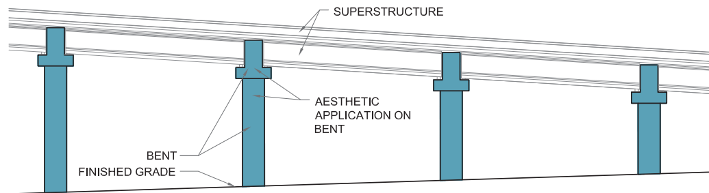
Figure 4.3 – Aesthetic treatment of bents in a sloping condition
