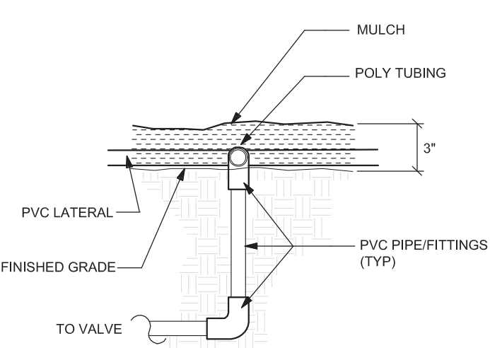
Figure 10.5– Typical irrigation PVC/header connection
