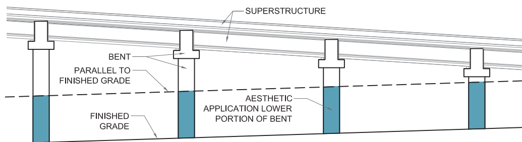
Figure 4.5 – Bents in a sloping condition with aesthetic treatment justified at the bottom.
