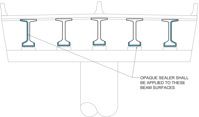
Figure 3.3 – Required surfaces for aesthetic treatment on concrete beams
