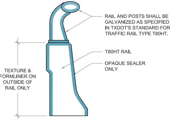
Figure 1.2 – Required aesthetic surface treatments on T80HT rails
