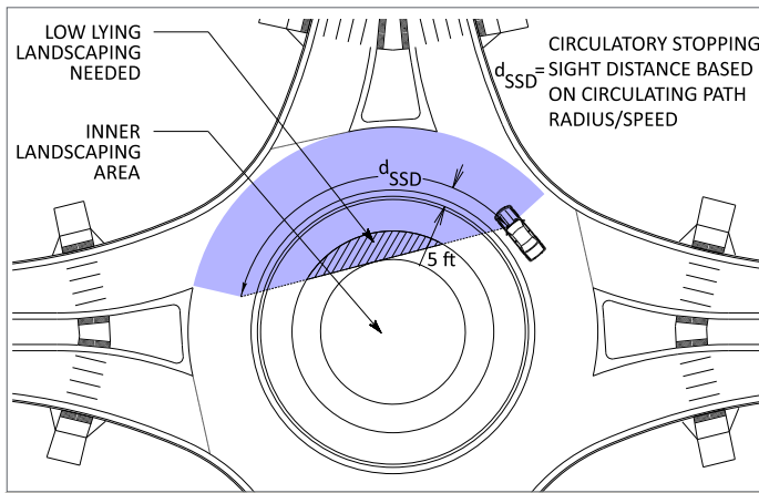
» FIGURE 44 – Circulating Stopping Sight Distance
