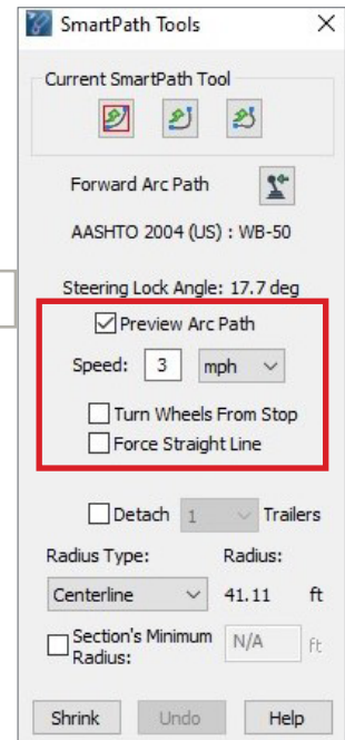
» FIGURE 31 – SmartPath Tool Dialog Box
