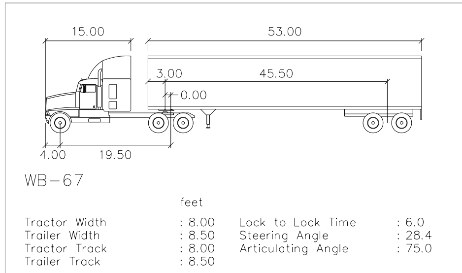
» FIGURE 39 – Example Truck Profile
