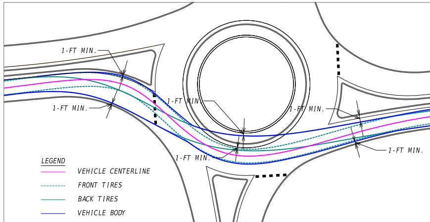
» FIGURE 29 – Offsets to Face of Curb
