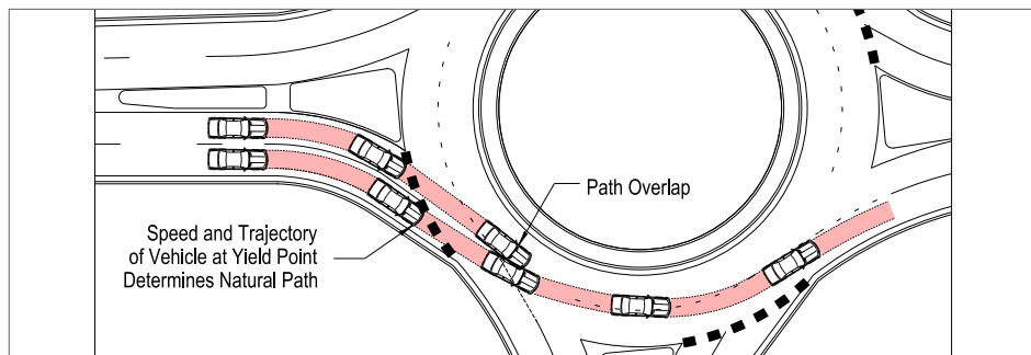
» FIGURE 1 – Path Overlap
