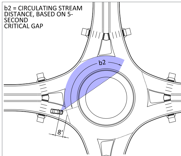
CIRCULATING INTERSECTION SIGHT DISTANCE
