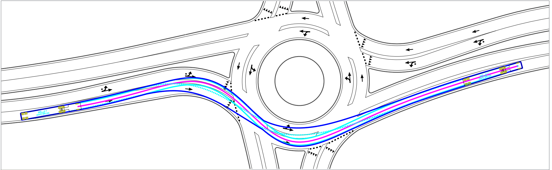
» FIGURE 36 – Straddle Lanes Design: Through Movement
