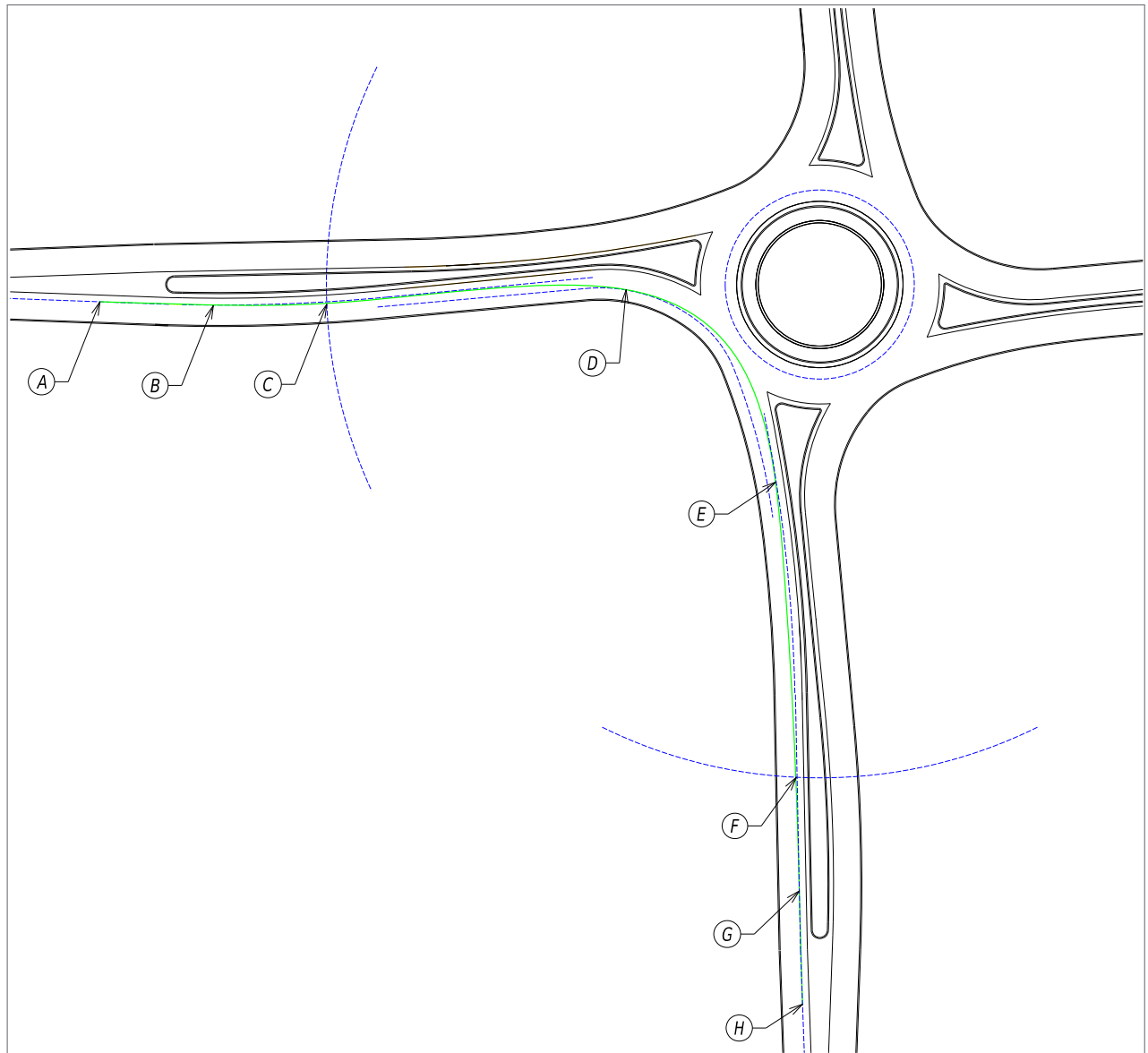
» FIGURE 10 – Typical Point Placement on a Right-Turn Spline
