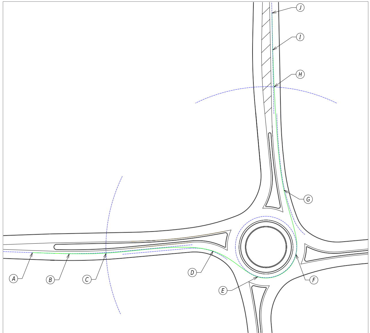
» FIGURE 9 – Typical Point Placement on a Left-Turn Spline
