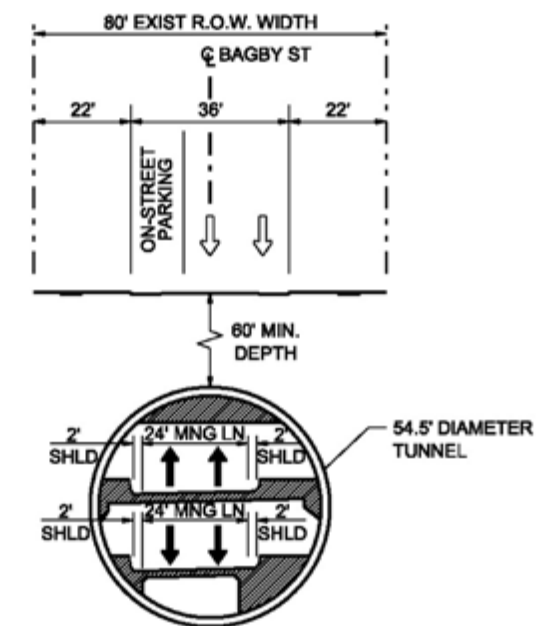
PROPOSED TYPICAL SECTION - BAGBY (ALTERNATIVE 7)
