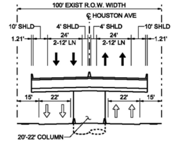
PROPOSED TYPICAL SECTION - HOUSTON (ALTERNATIVE 8A)
