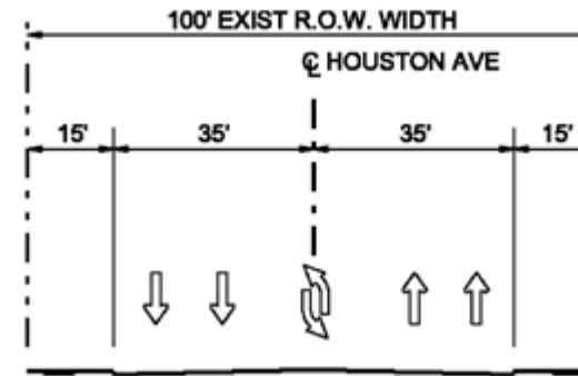
EXISTING TYPICAL SECTION - HOUSTON
