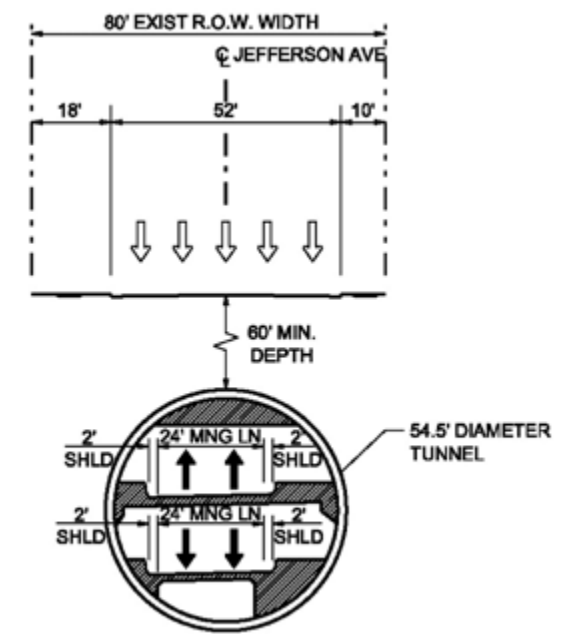
PROPOSED TYPICAL SECTION - JEFFERSON (ALTERNATIVE 7)
