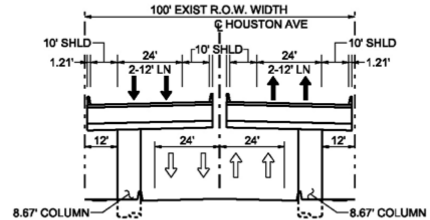
PROPOSED TYPICAL SECTION - HOUSTON (ALTERNATIVE 8B)
