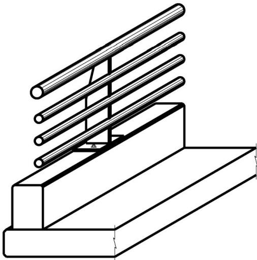
Figure A–16. Type PR22 Railing
