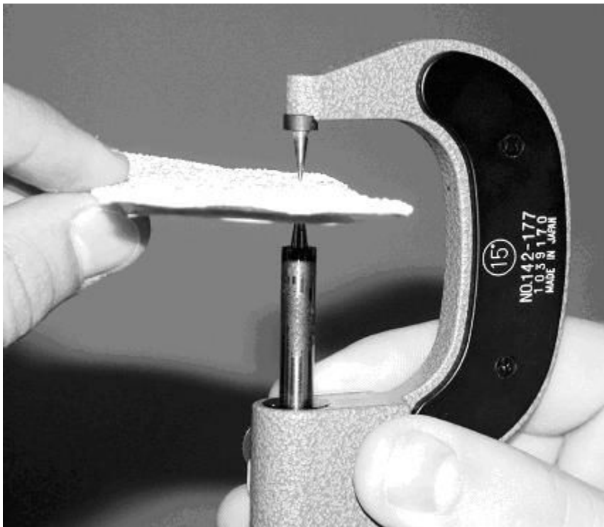
Figure 3-1. Needlepoint micrometer measuring thermoplastic sample.
