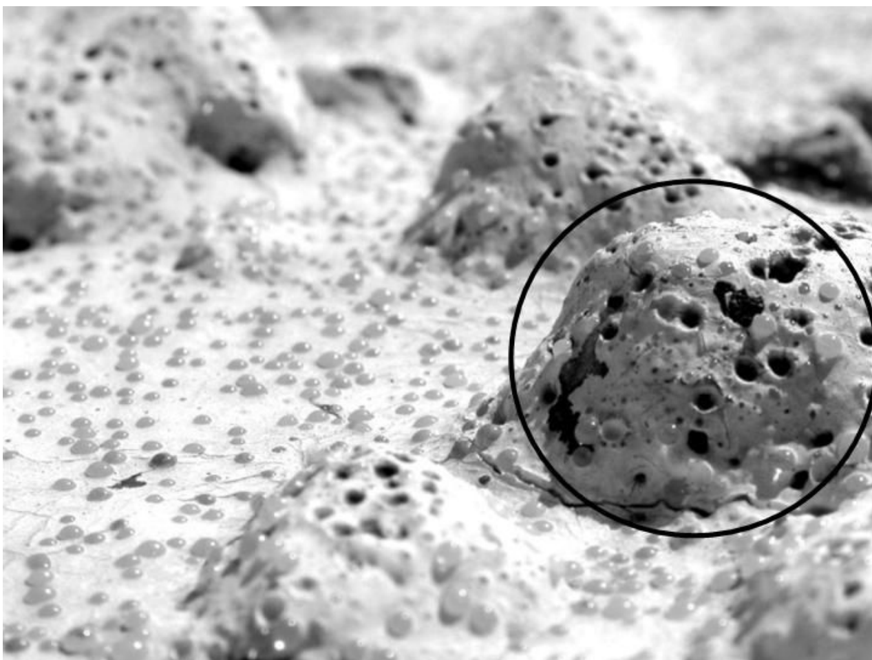
Figure 2-5. Poor bead retention on top of aggregates.
