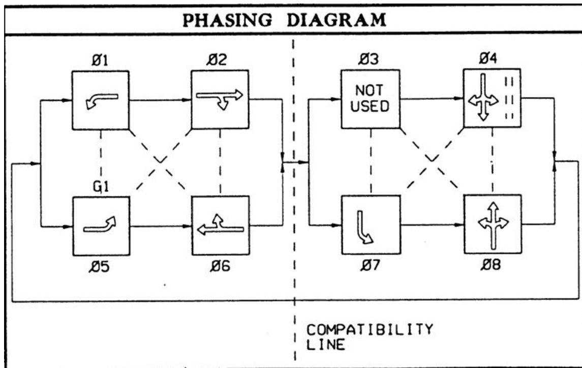
Figure 5-1. Typical phasing diagram.
